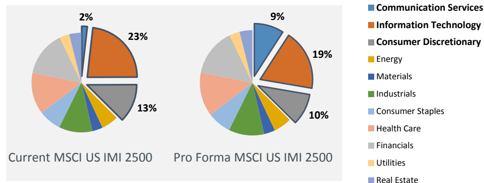
Sector Weight Impact on MSCI US Inv. Market 2500*
